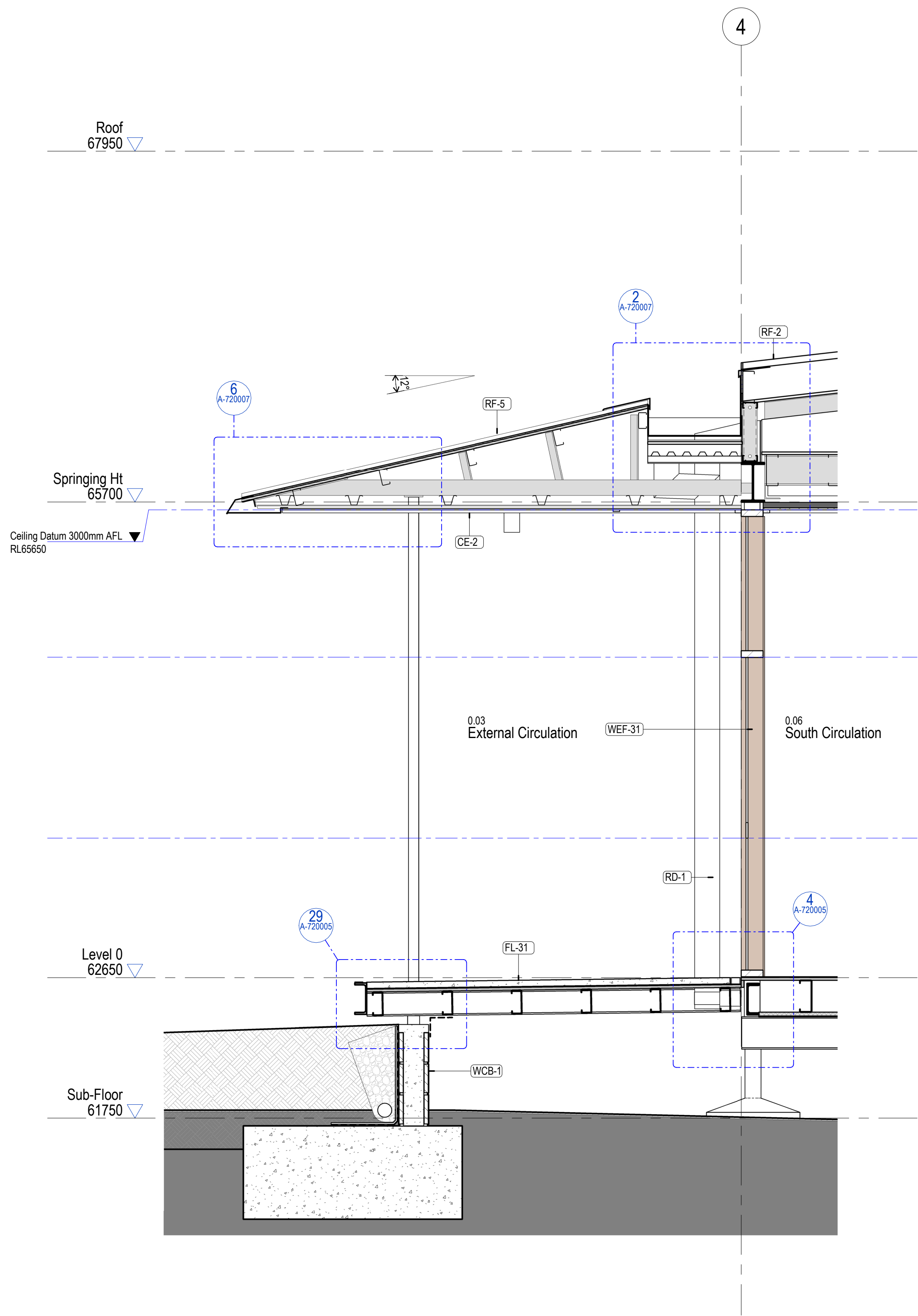
1 Courtyard South Facade Section 1 : 20
